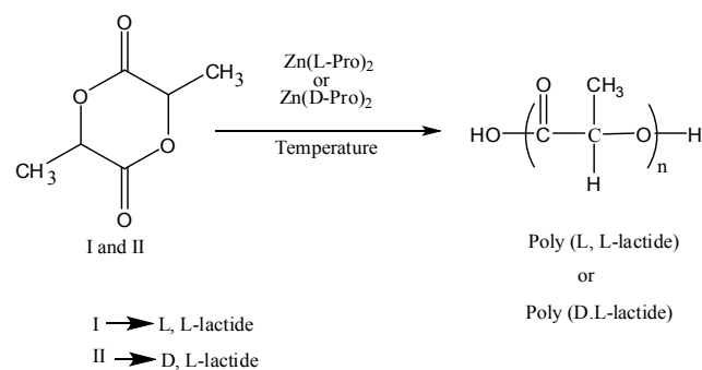
Fig. 2. Homopolymerization of L, L-lactide and D, L-lactide.
