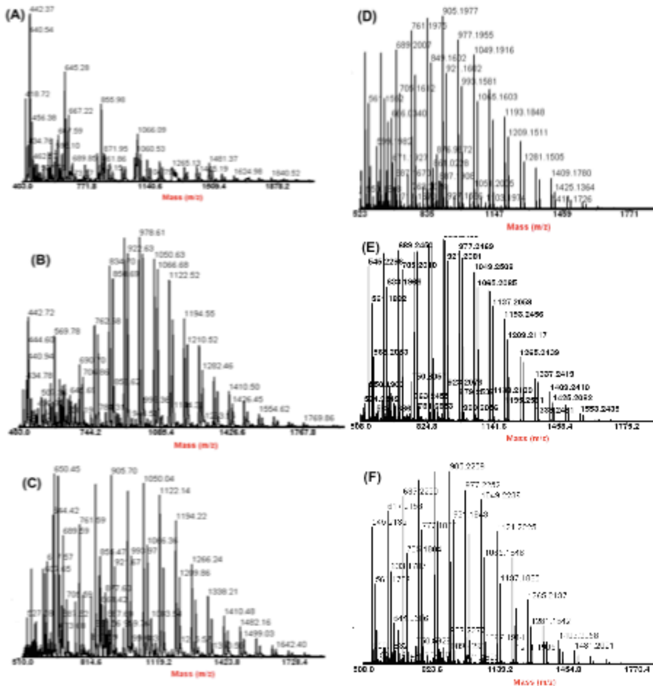
Fig. 6. (A) MALDI ToF-MS of L-3 oligomers, (B) MALDI ToF-MS of L-5 oligomer, (C) MALDI ToF-MS of L-9 oligomer, (D) MALDI ToF-MS of L-13 oligomer, (E) MALDI ToF-MS of L-14 oligomer and (F) MALDI ToF-MS of L-15 oligomer.
