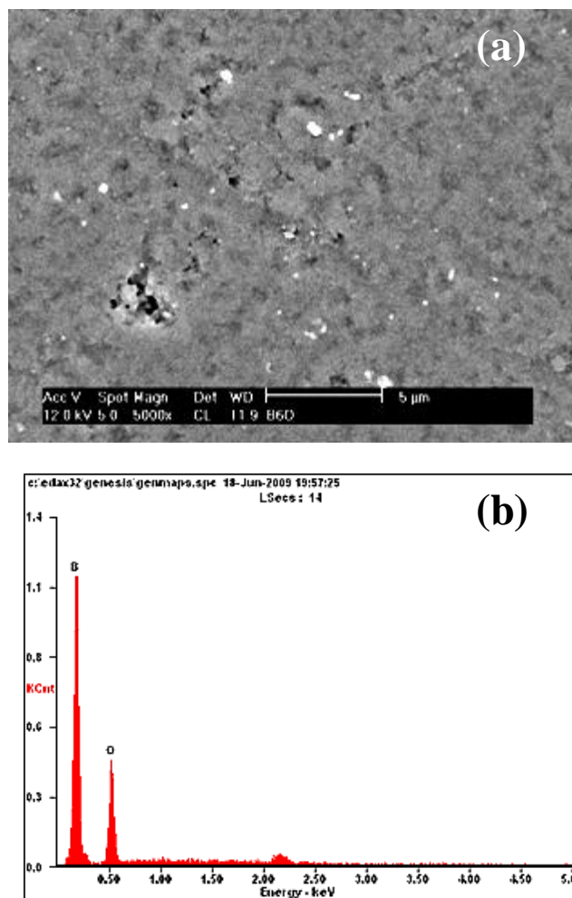
Fig. 1. Shows the SEM surface micrograph (a) and the EDX surface compositional analysis (b) of a hot pressed B 6 O specimen. Iron contamination is responsible for EDX elemental peak observed around 2.25 keV.
