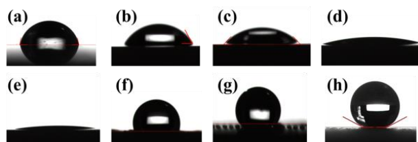
Fig. 7. Photographs of the water droplets on the (a) polished sample, (b) textured surface, (c) PDA modified surface, (d) PDA and textured surface, (e) PDA and textured surface with copper particles, (f) DT modified surface with copper particles, (g) DT modified surface with texture and (h) DT modified surface with texture and copper particles.
