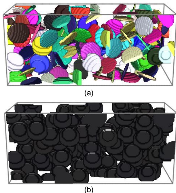
Fig. 5. 173 flakes in (a) random distribution and (b) aligned along the direction of electric field.
