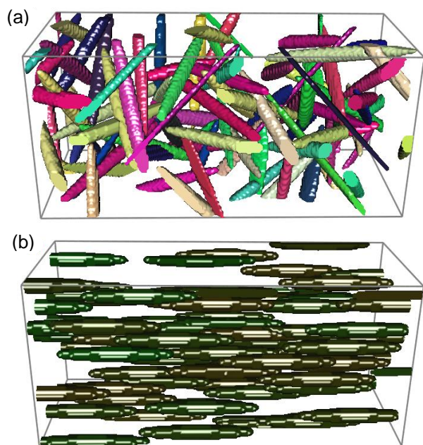
Fig. 2. 100 rods with a total volume fraction 10.42% in a matrix: (a) in random distribution; (b) aligned along the direction of electric field.
