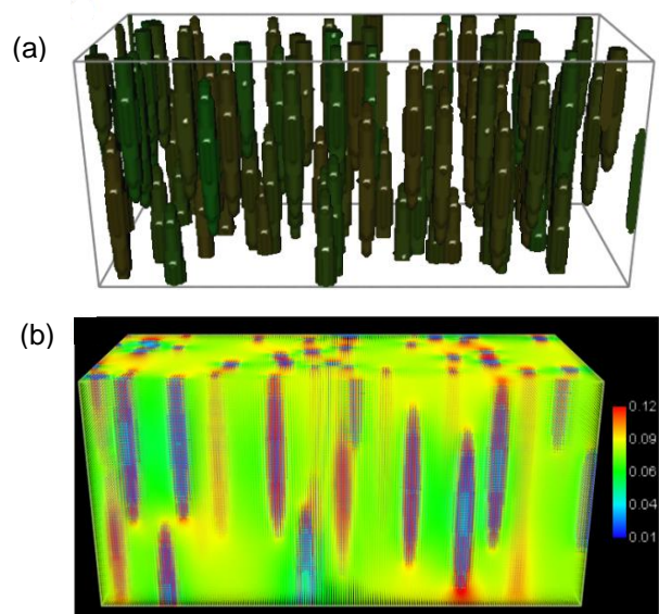
Fig. 4. (a) 100 rods are aligned to a direction in perpendicular to that of the electrical field and (b) the correspondence electric current density distribution.
