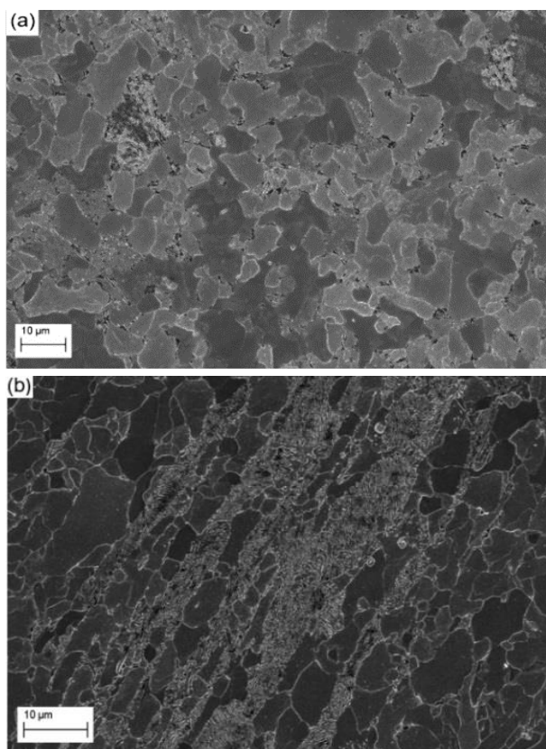
Fig. 1. Electric-field-induced alignment: (a) before and (b) after treatment.
