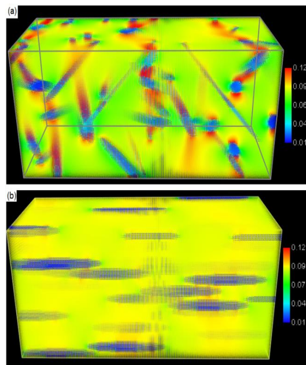
Fig. 3. The electric current density in a matrix containing 100 rods at (a) randomly distribution and (b) aligned along the direction of electric field.
